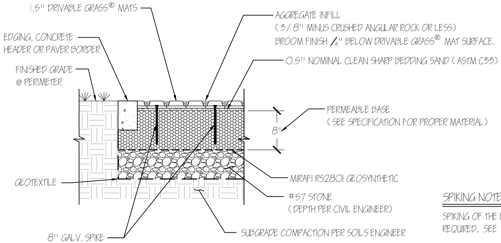
INFILL DETAIL
