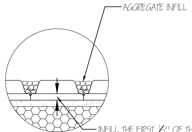
INFILL DETAIL
