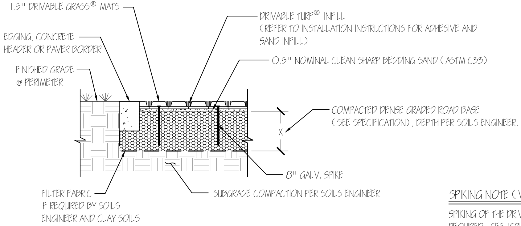
TYPICAL PROFESSIONAL DRIVABLE GRASS® DETAIL WITH DRIVABLE TURF® INFILL
