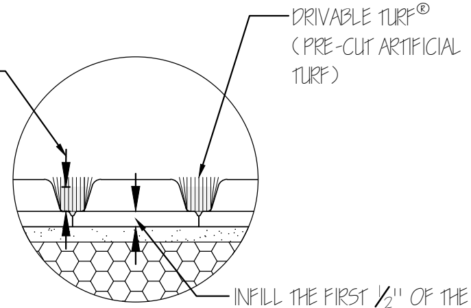
INFILL DETAIL INFILL THE FIRST 1/2" OF THE DRIVABLE GRASS® MATS WITH BEDDING OR #30 SAND.
