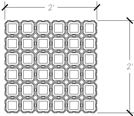
DRIVABLE GRASS® CONCRETE MAT
