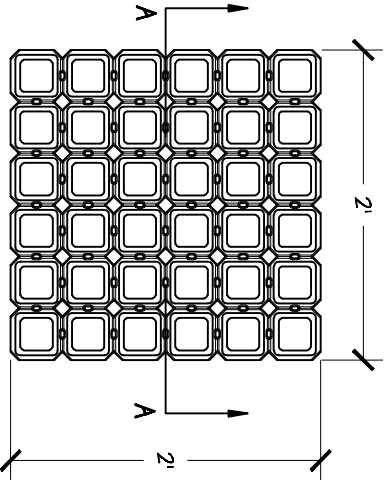
PLAN VIEW
